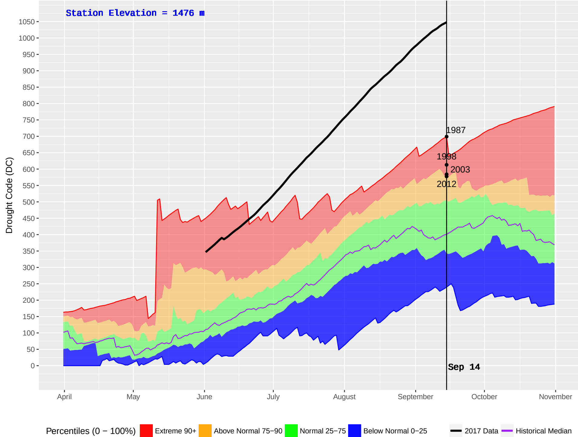
BRENDA MINES (283) : Historical (1977–2016) and Current (2017) Noon Drought Code (DC)
